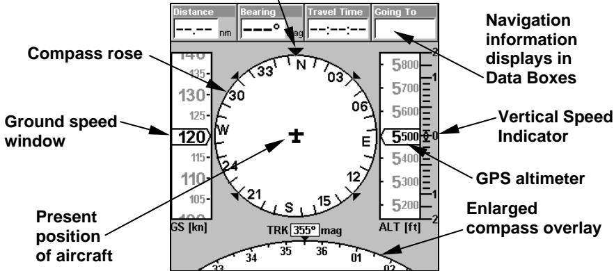
Navigation Panel Page, traveling north. Page looks like this when AirMap is not navigating to a waypoint, following a route, or backtracking a trail.
